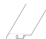
End Cap 1" x 0.4" x 94.5"
