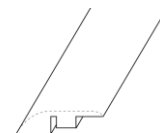
Reducer 1.8" x 0.4" x 94.5"
