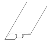
Reducer 1.8" x 0.4" x 94.5"
